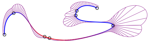
Fig. 9. An example curve generated with hybrid interpolation function, showing that the local curvature maxima appear near control points. The purple lines indicate the curvature of the curve.
