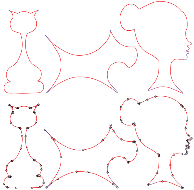
Fig. 15. Examples curves generated using the hybrid interpolation function, showing sharp features achieved by placing control points in close proximity. Artwork by Ozum Yuksel .
