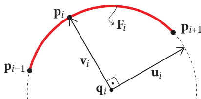
Fig. 6. The affine-invariant representation of the circular interpolation function.
