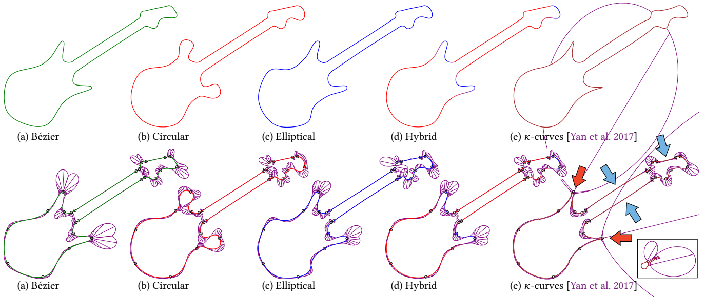
Fig. 13. Comparison of (a-d) curves generated using our method with four example interpolation functions and (e) \kappa -curves [Yan et al. 2017] from the same control points. The bottom row shows the control point positions and the curvature of the curves. The inset on the right bottom provides a zoomed-out view, showing the entire curvature visualization of \kappa -curves. The red arrows highlight the extremely sharp corners generated by \kappa -curves and the blue arrows show the curve segments that are bent due to the global support of \kappa -curves.
