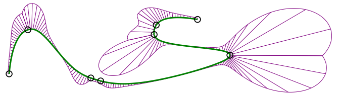
Fig. 4. An example curve generated with Bézier interpolation function, showing that the local curvature maxima appear near control points. The purple lines indicate the curvature of the curve.
