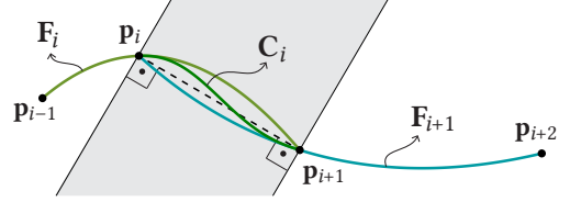
Fig. 3. The curve generated with Bézier interpolation function remains between two control points (the shaded region).
